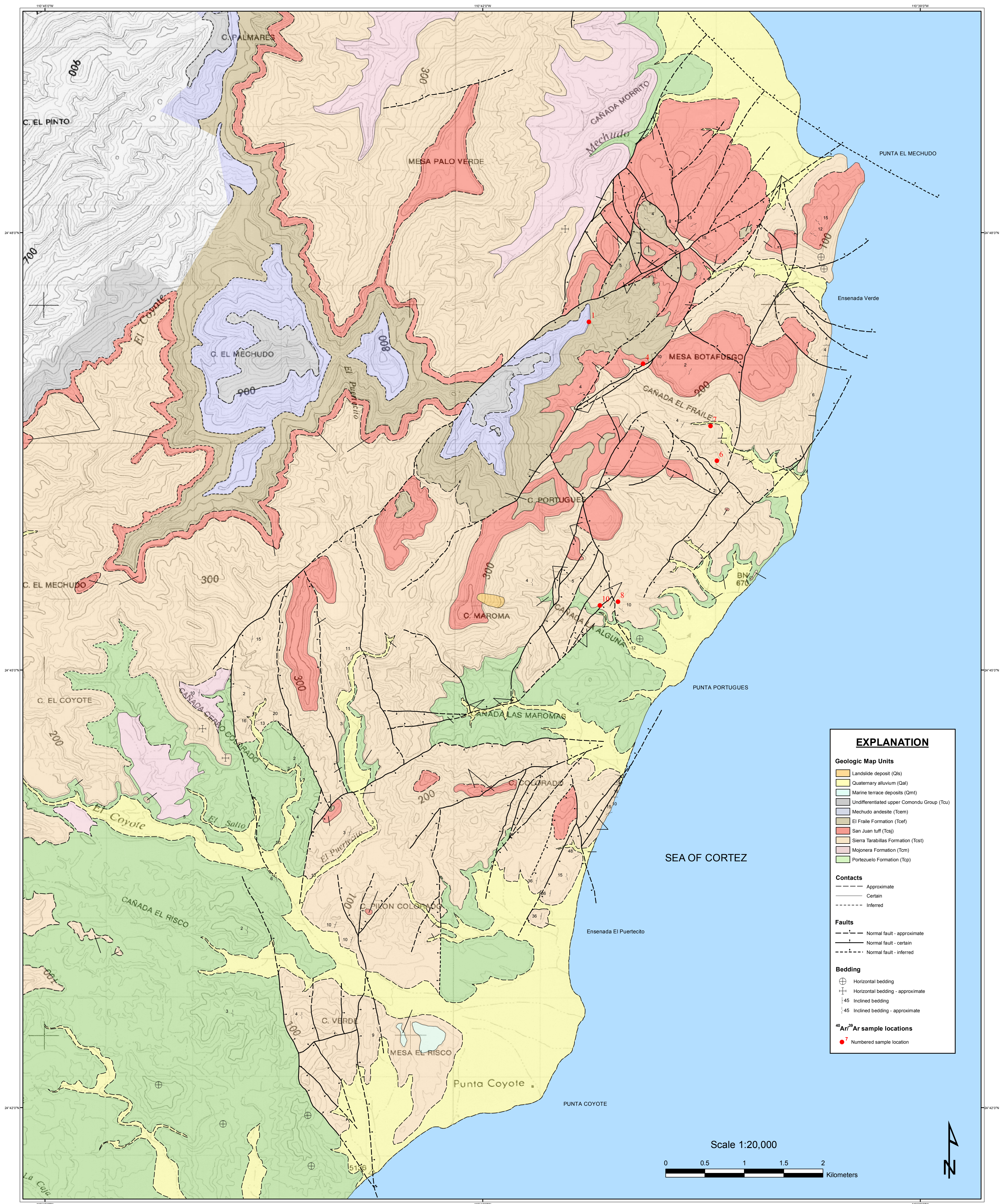
Plate 6. Geologic map of the Cerro El Mechudo area, Baja California Sur, Mexico
