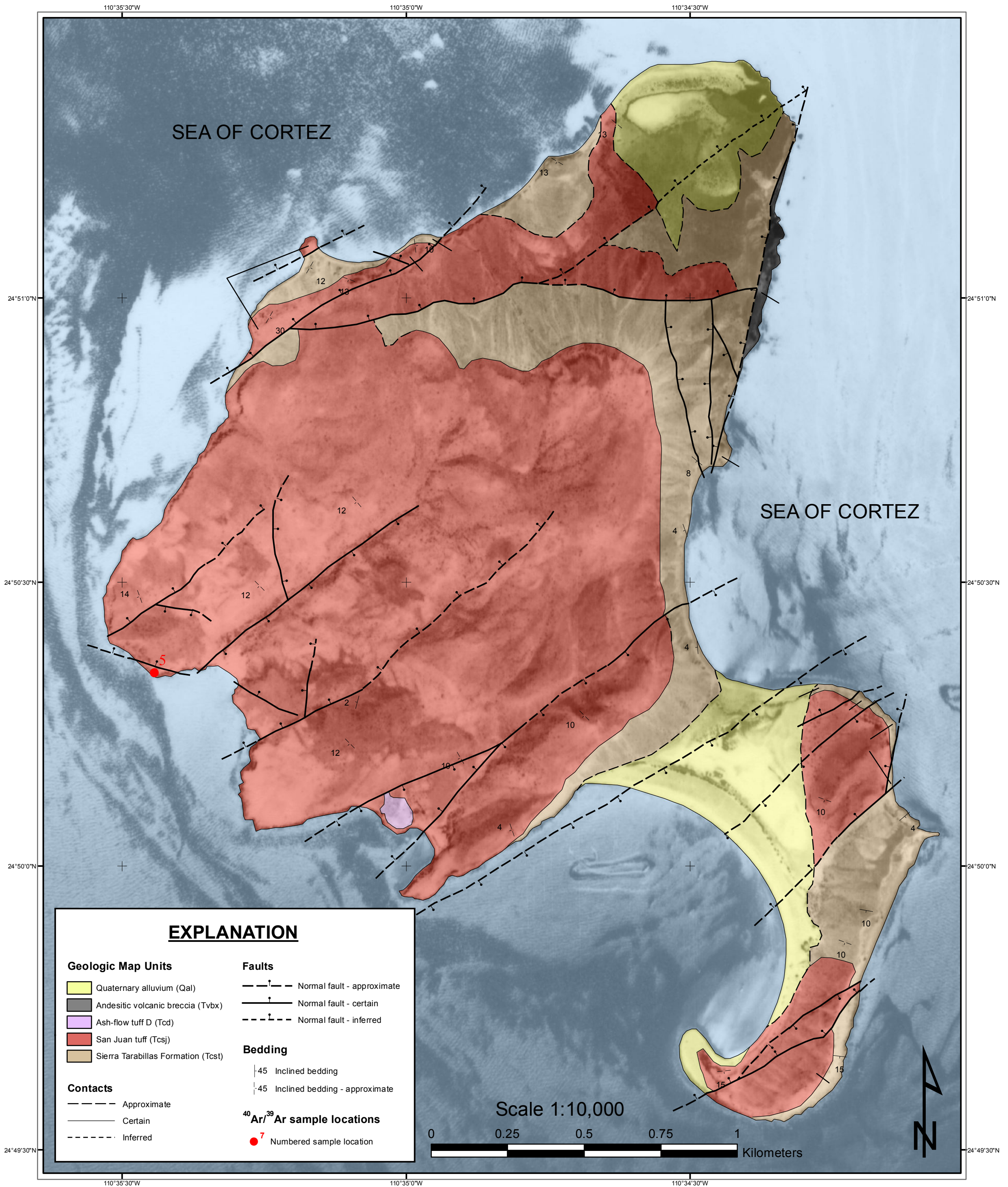
Plate 4. Geologic map of San Francisquito Island, Baja California Sur, Mexico
