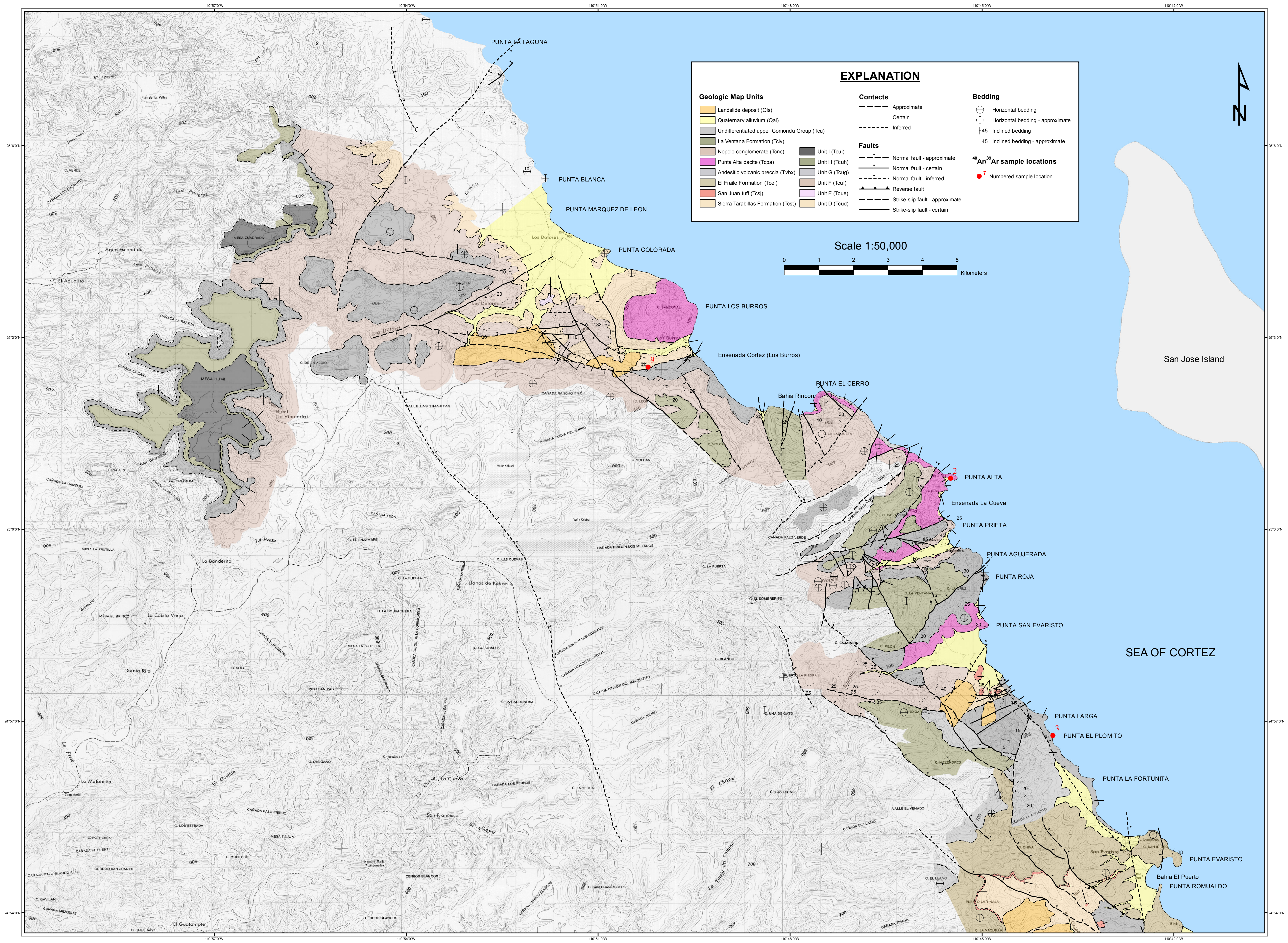
Plate 3. Geologic map of the San Evaristo, Punta Alta, and Los Burros area, Baja California Sur, Mexico
