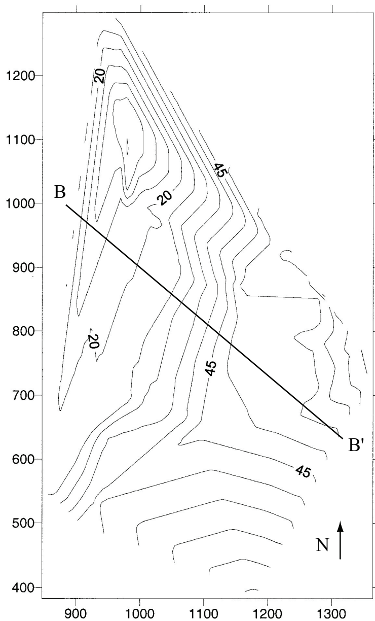
Figure 4.8: Elevation contour map of Bahia Marquer survey area #2. All dats are relative to an arbitrary point. The 25 m (125 ka) terrace and 55 m terrace are visible. Cross-section B to B' is shown in figure 4.9.
