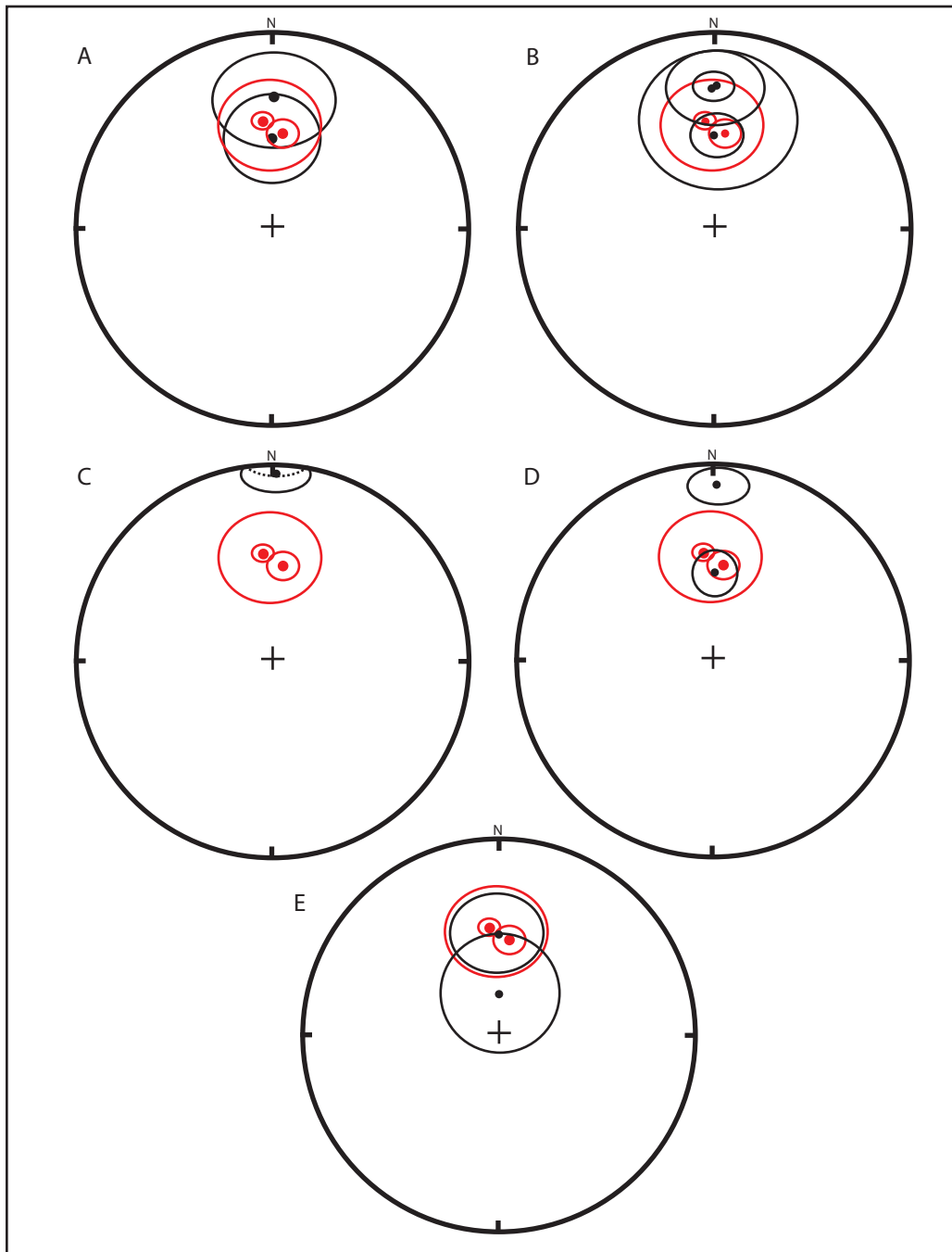
Figure 3.18: Stereonet plot of the paleomagnetic samples from Carmen Island after they have been rotated counterclockwise back to reference sample on San Javier road. Plot compares inclinations if all samples had similar declination. San Javier road is plotted in red and 95% confidence between San Javier sites is larger red circle. All 95% confidence cones are shown as circles surrounding individual points. A) Sample from middle-west paleomagnetic domain on Carmen Island. B) Sample from middle-east paleomagnetic domain. C) Samples from southwest paleomagnetic domain. D) Samples from southeast paleomagnetic domain. E) Samples from northern Pliocene paleomagnetic domain.
