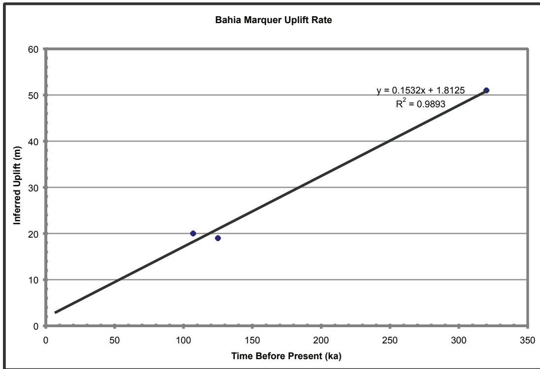
Figure 4.21: Inferred uplift versus time at Bahia Marquer. Equation besides curve is determined from linear regression analysis and indicates an average uplift rate of \sim 0.15 m/ka.
