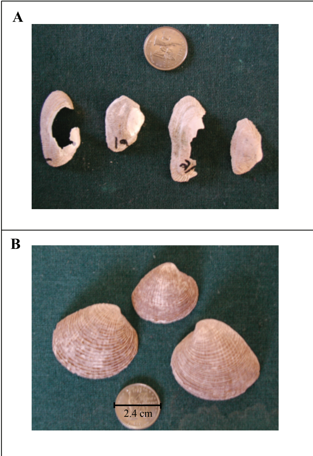
Figure 4.15: Two types of shell species from Bahía Marquer and Punta El Bajo. A) Cardita californica , found on 25 m (125 ka) terrace at Bahía Marquer. B) Chione californiensis , found on 18 m (107 ka) terrace at Bahía Marquer and 6 m (107 ka) terrace at Punta El Bajo.
