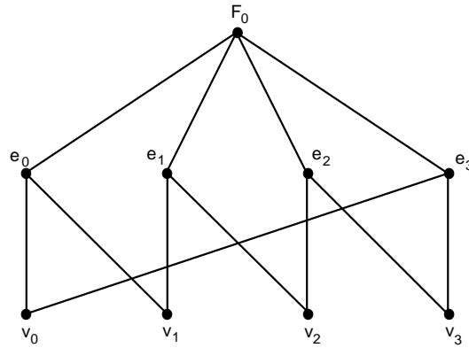
Figure 1.3: Face poset for a regular cell complex
