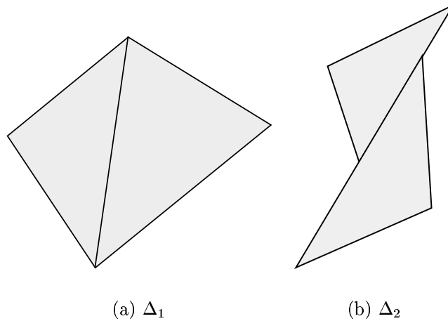
Figure 1.4: Collections of simplices
