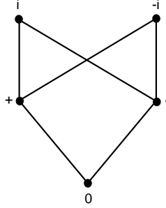
Figure 5.5: The partial ordering on \{0, +, -, i, -i\}
