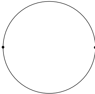
Figure 1.1: S^1 as a regular cell complex
