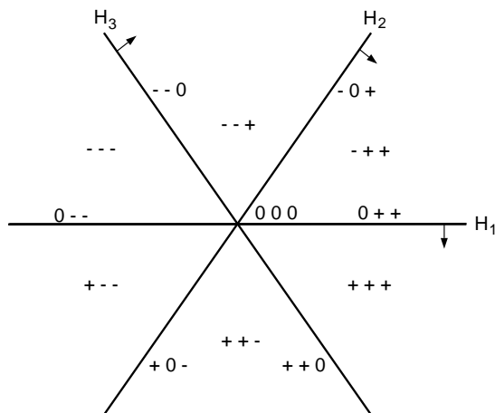
Figure 4.1: Covectors of \mathcal{A}_2
