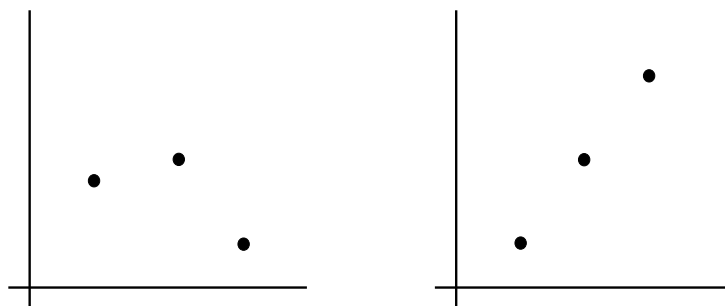
Figure 6.1: Unlabelled point configurations of F_3(\mathbb{C})
