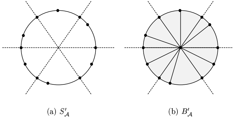
Figure 2.5: Simplicial decomposition of S^1 and B^2
