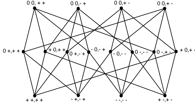
Figure 5.2: Poset for \text{Sal}(\mathcal{A})
