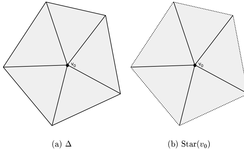
Figure 1.5: The star of a vertex
