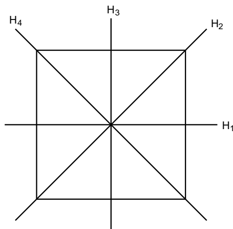
Figure 3.1: A finite reflection arrangement of type B_2
