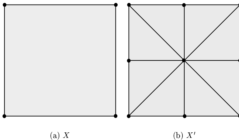
Figure 1.7: Barycentric subdivisions of a regular cell complex
