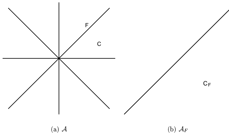
Figure 2.4: A subarrangement
