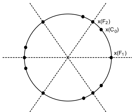
Figure 3.3: W -invariant S'_{\mathcal{A}}
