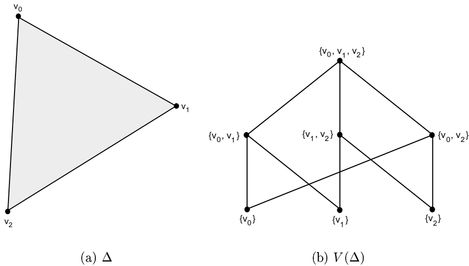
Figure 1.6: A simplicial complex and its vertex scheme
