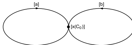
Figure 6.4: The orbit complex |\text{Sal}(\mathcal{A}_2)|/S_3
