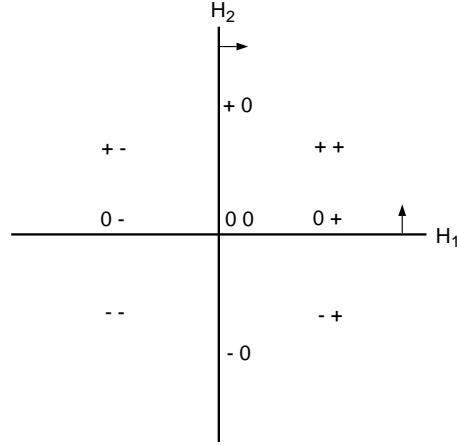
Figure 5.1: Covectors of a hyperplane arrangement
