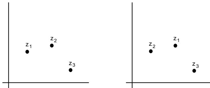
Figure 3.5: Labelled point configurations of \hat{F}_3(\mathbb{C}) .
