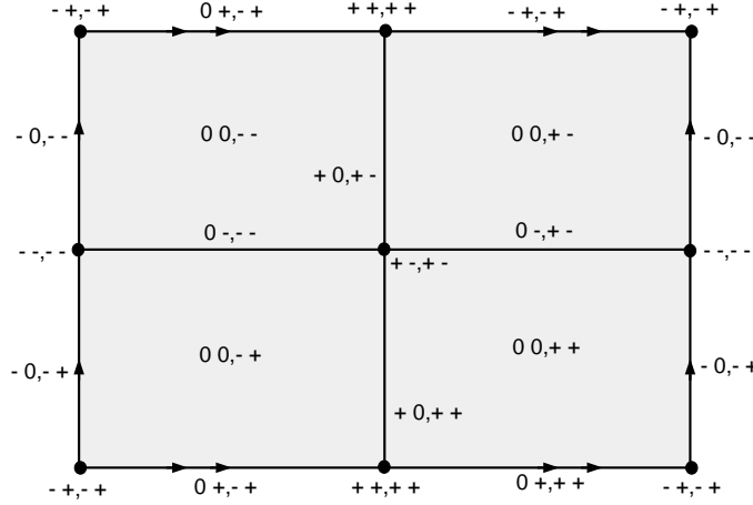
Figure 5.3: A realization of \text{Sal}(\mathcal{A})
