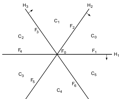
Figure 2.2: Faces of a hyperplane arrangement
